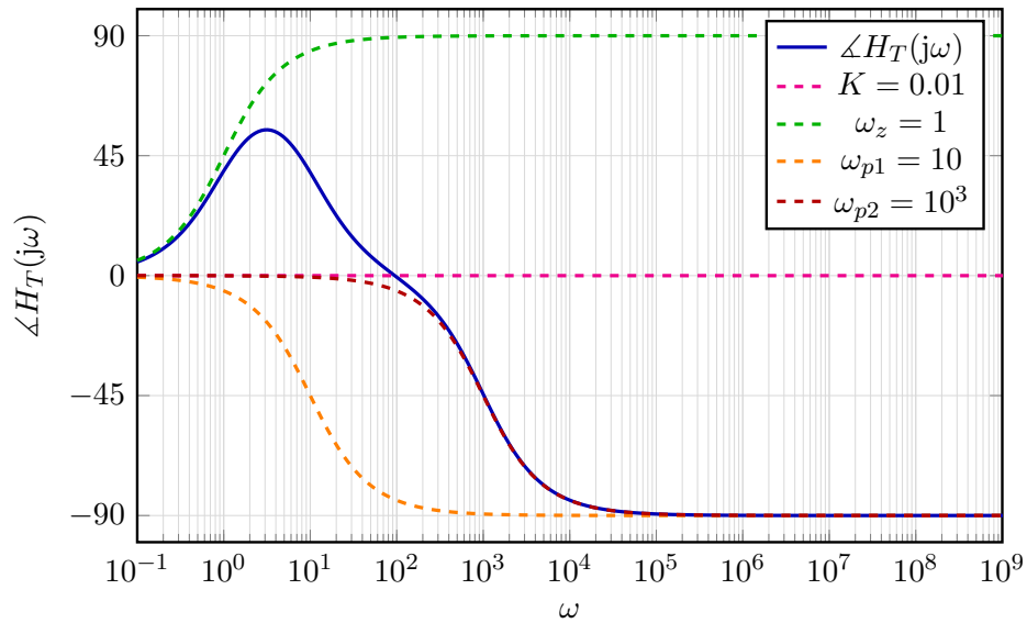
Figure 15: Phase Bode Plot of H_T(j\omega)
