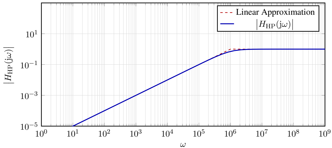
Figure 5: High-pass filter magnitude plot.
