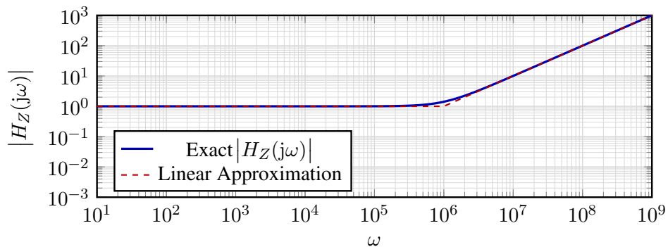
Figure 9: Simple Zero, Magnitude Plot.
