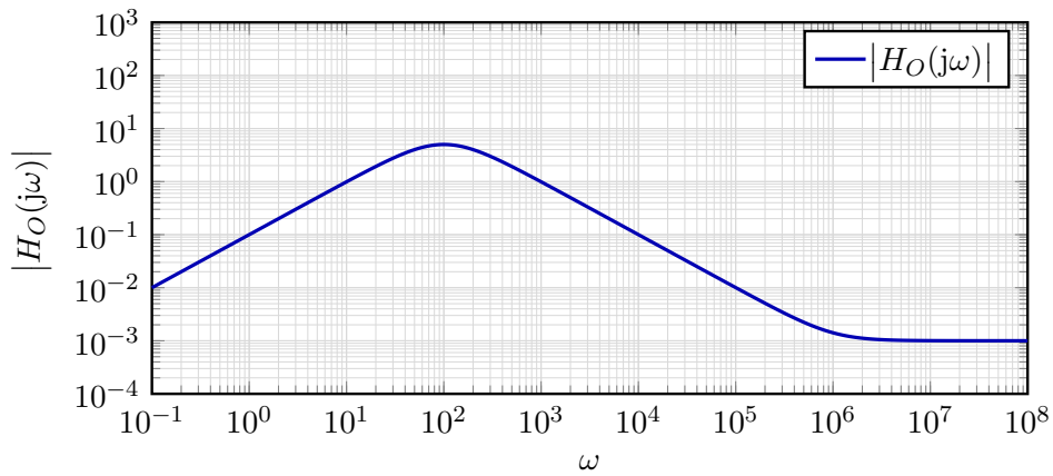
Figure 16: Magnitude Bode Plot of H_O(j\omega)
