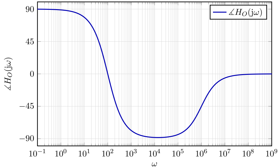
Figure 17: Phase Bode Plot of H_O(j\omega)
