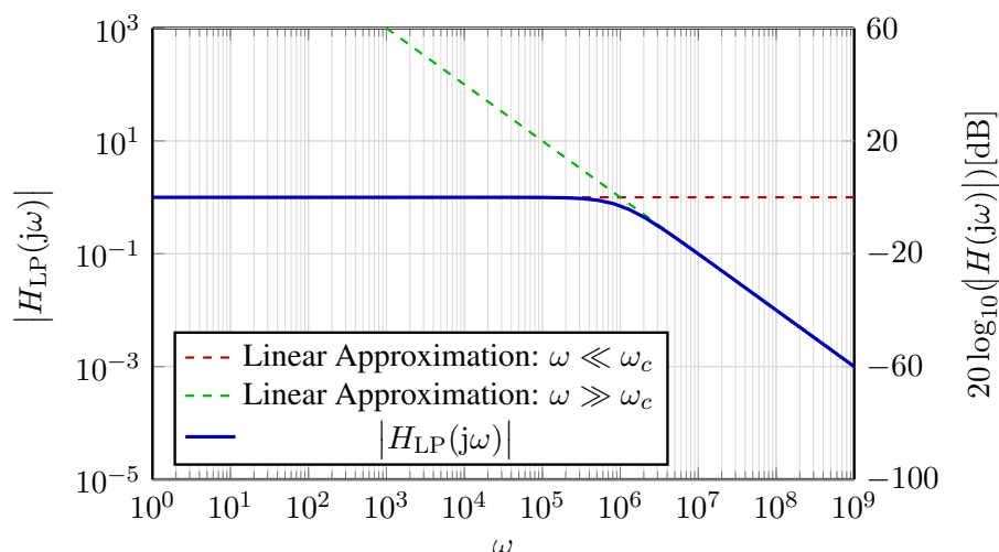
Figure 1: Low-pass filter magnitude plot, with 2 asymptotes drawn (dashed).
