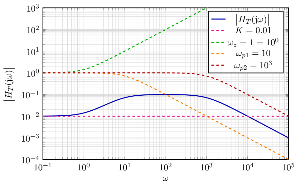
Figure 14: Magnitude Bode Plot of H_T(j\omega)
