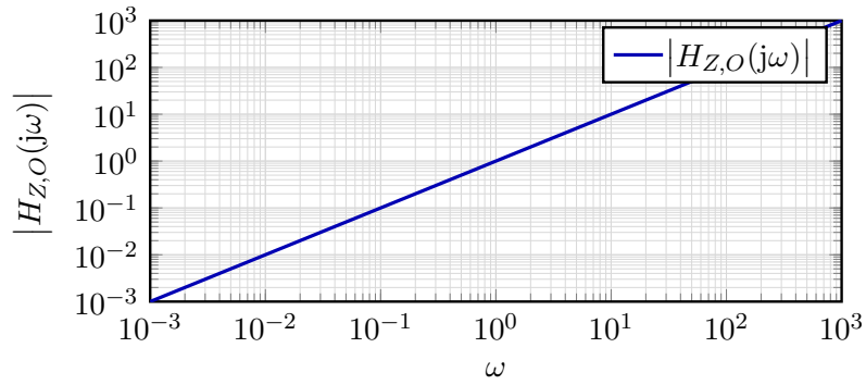
Figure 12: Origin Zero, Magnitude Plot.
