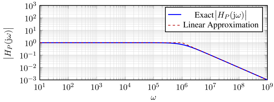
Figure 7: Simple Pole, Magnitude Plot.
