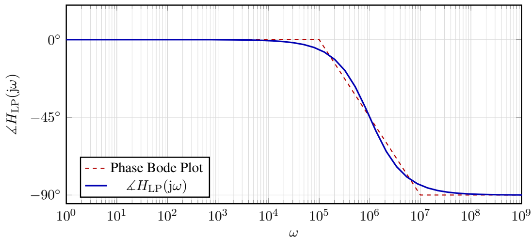
Figure 4: Low-pass filter phase plot.
